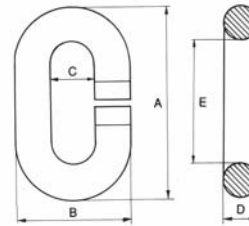
SPLIT LINK
